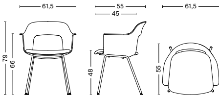
LAYOUT ARMCHAIR 214 Width 62 cm Depth 56 cm Height 80 cm Seat height 48 cm Armrest height 67 cm Weight 8,95 kg
