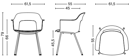
LAYOUT ARMCHAIR 211 Width 61,5 cm Depth 55 cm Height 79 cm Seat height 45,5 cm Armrest height 66 cm Weight 7,45 kg
