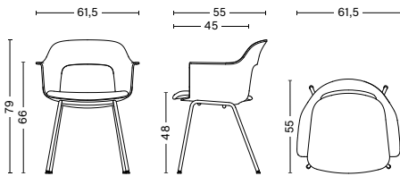
LAYOUT ARMCHAIR 213 Width 61,5 cm Depth 55 cm Height 79 cm Seat height 48 cm Armrest height 66 cm Weight 8,05 kg
