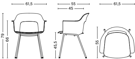
LAYOUT ARMCHAIR 212 Width 61,5 cm Depth 55 cm Height 79 cm Seat height 45,5 cm Armrest height 66 cm Weight 7,15 kg
